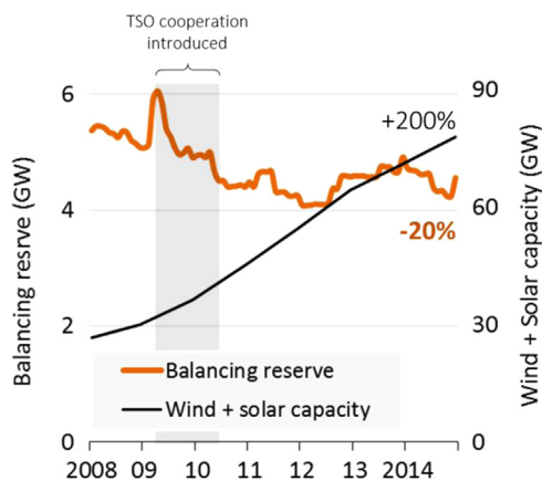
Fig. 7. Balancing reserves (SC+TC, average of positive and negative reserve) and VRE capacity (wind + solar) in Germany. Even though the installed capacity of wind and solar power has tripled since 2008, the demand for balancing power has decreased. One reason was the cooperation between TSOs introduced in 2009/2010.
