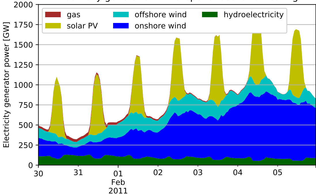
Electricity generation in Europe for scenario Heating
