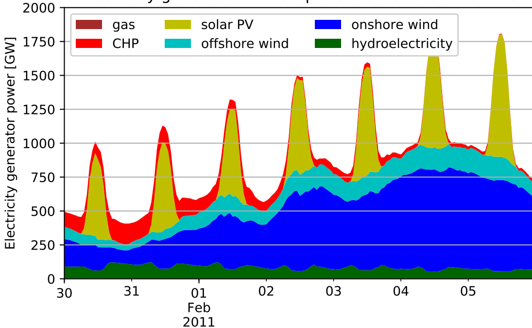
Electricity generation in Europe for scenario Central-TES
