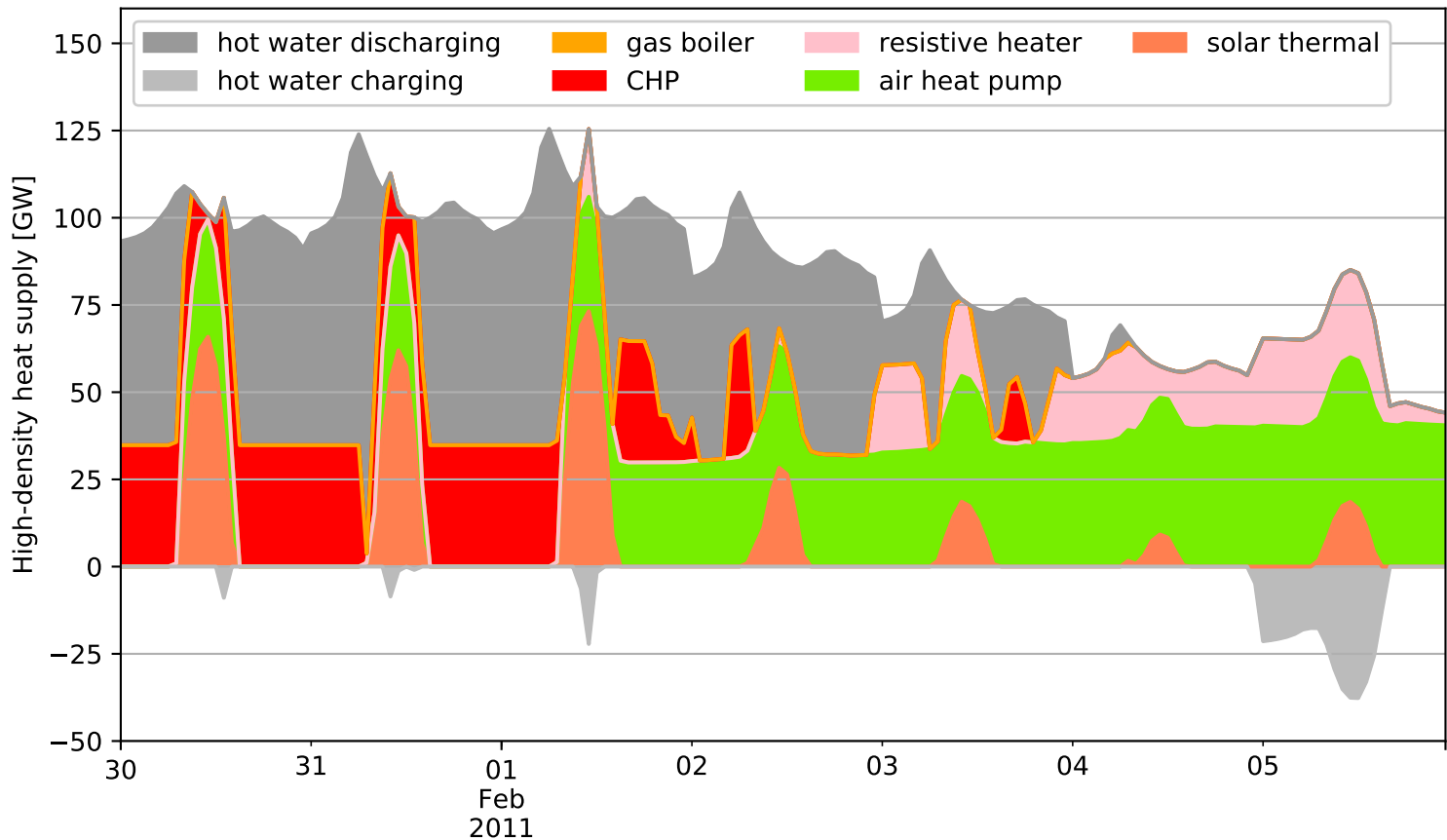
High-density heat supply in DE for scenario Central-TES
