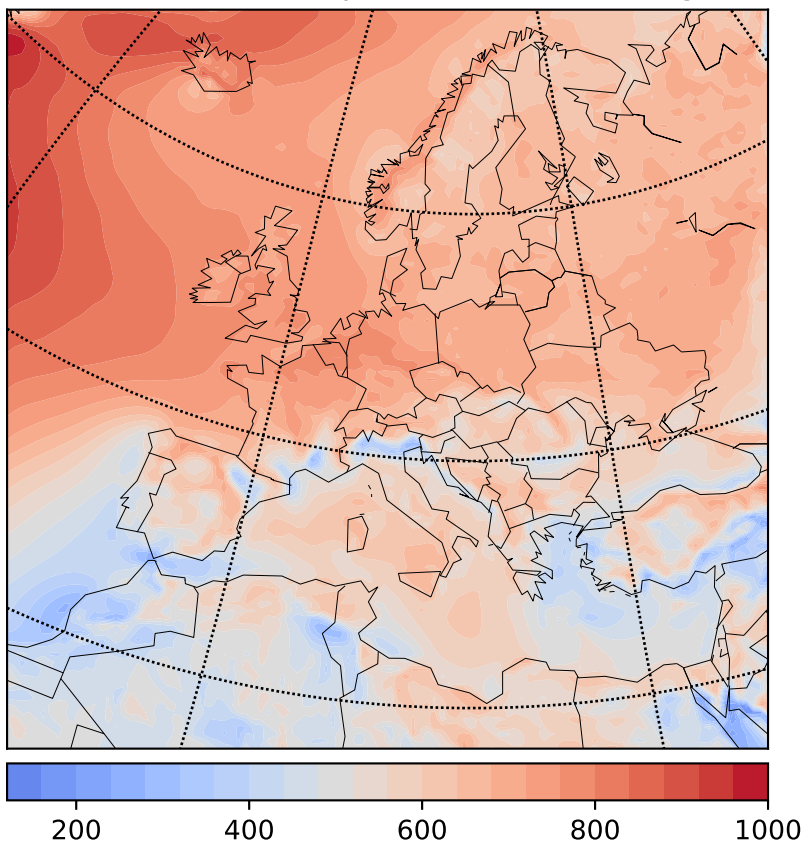
Ensemble Mean - Wind Speed Correlation Length - moc
