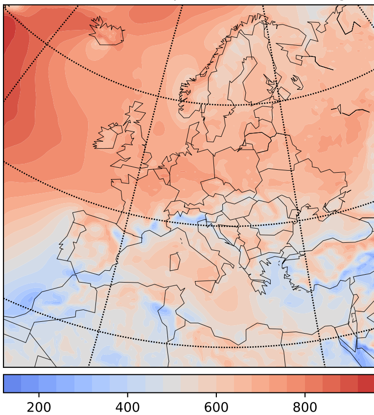
Ensemble Mean - Wind Speed Correlation Length - his
