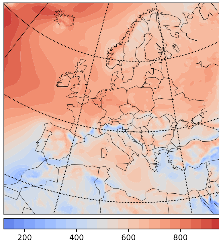
Ensemble Mean - Wind Speed Correlation Length - boc
