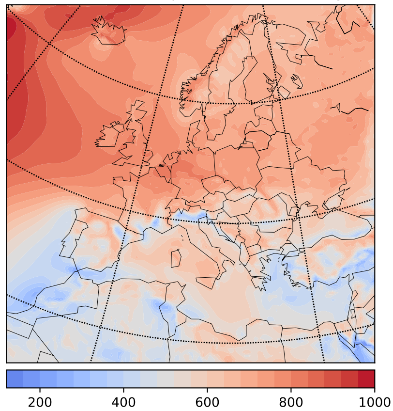
Ensemble Mean - Wind Speed Correlation Length - eoc
