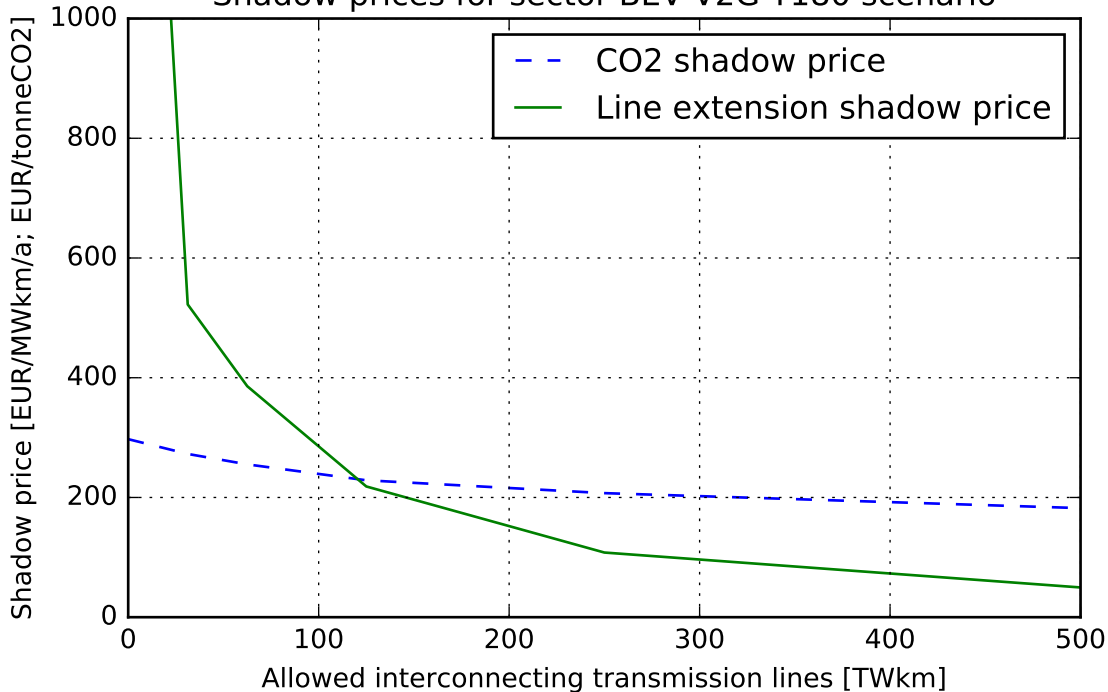
Shadow prices for sector BEV V2G T180 scenario
