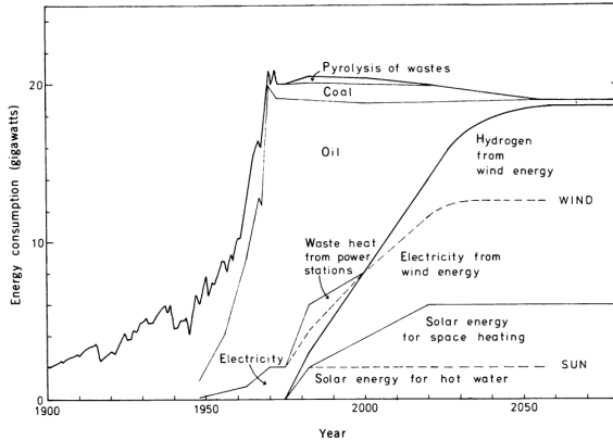
Fig. 4. Net energy consumption in Denmark, shown according to sources. Up to 1974, actual data are shown (I4); data after 1974 indicate the proposed plan. The relative weighting between solar and wind energy shares might be altered, for example, if a major breakthrough occurred in the development of solar cells, making them competitive to wind-produced electricity under Danish conditions. The heavy, solid line indicates the proposed total share of solar and wind energy.
