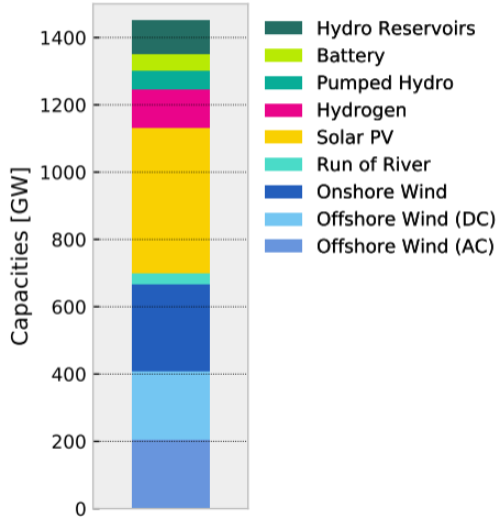
Optimal System Layout
