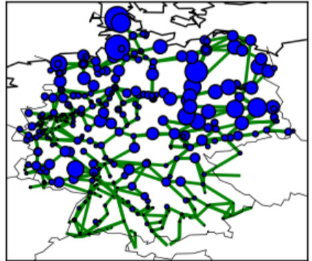
Wind Onshore
