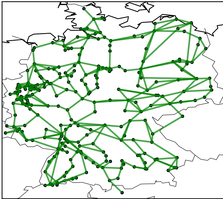
k-means: 422 -> 256
