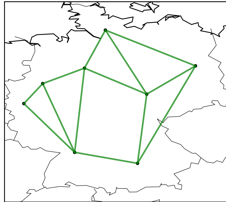
k-means: 422 -> 8
