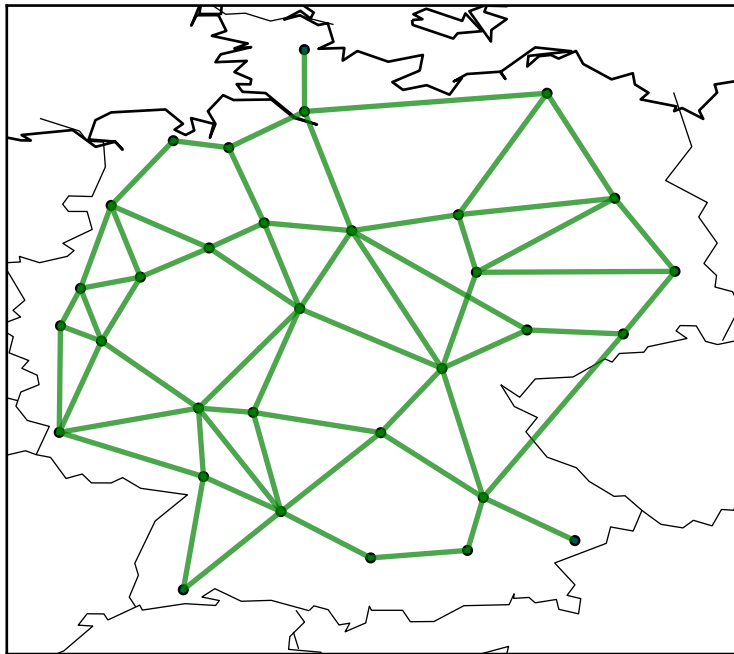
k-means: 422 -> 32
