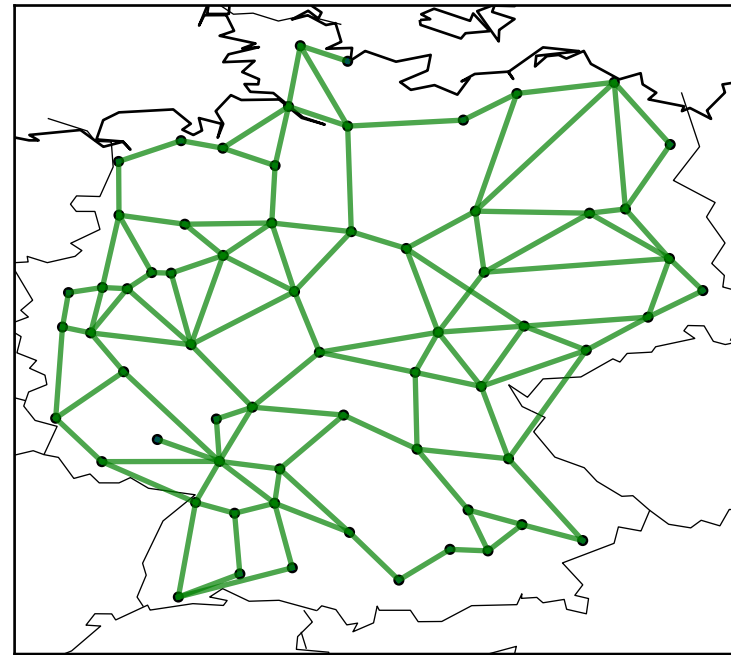
k-means: 422 -> 64
