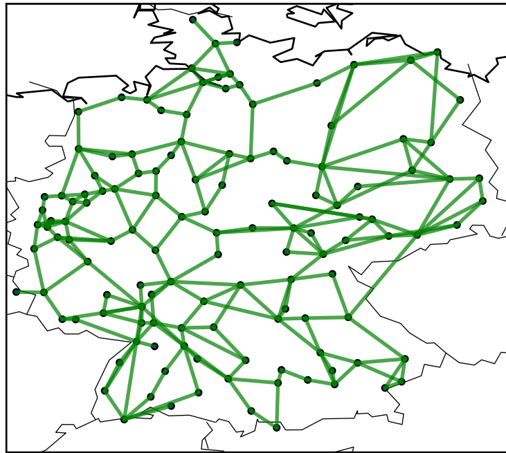
k-means: 422 -> 128
