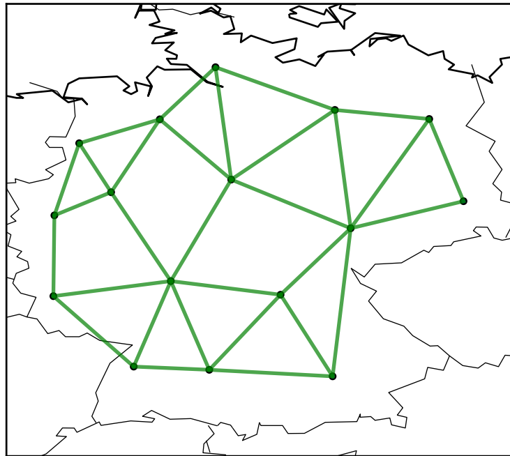
k-means: 422 -> 16
