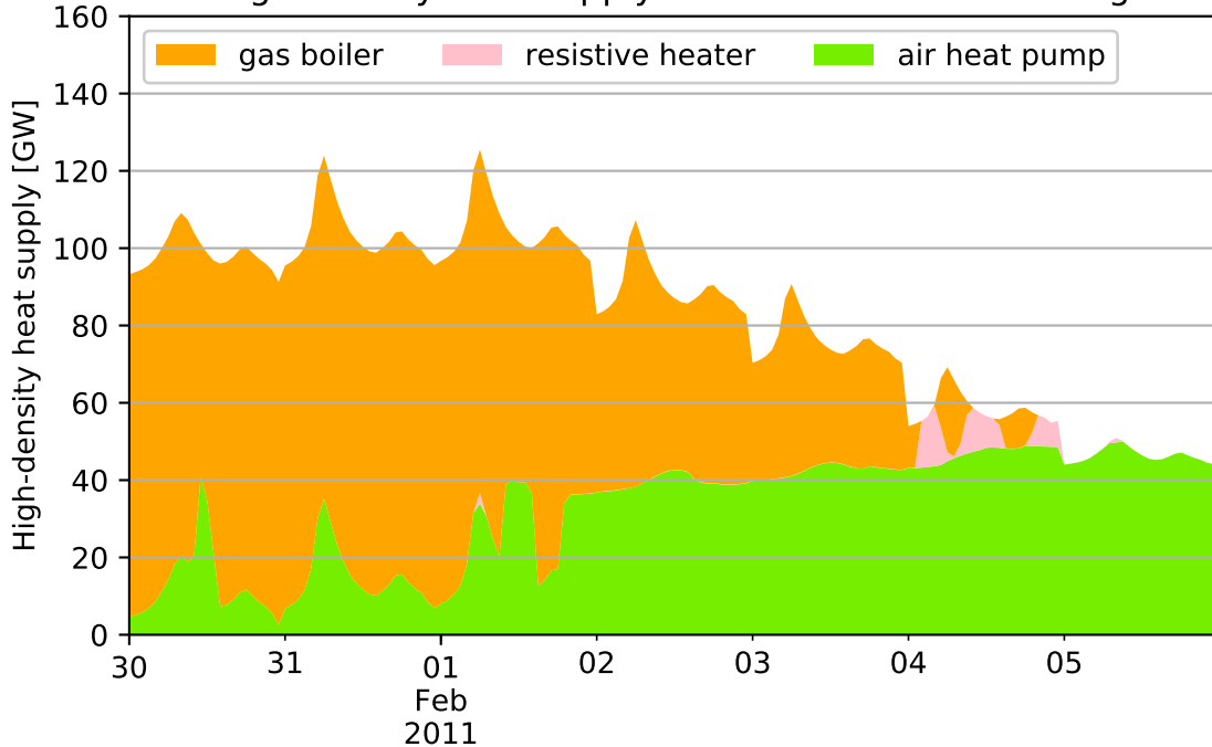
High-density heat supply in DE for scenario Heating
