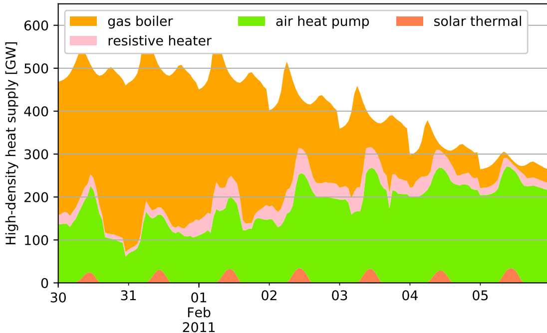
High-density heat supply in Europe for scenario Heating
