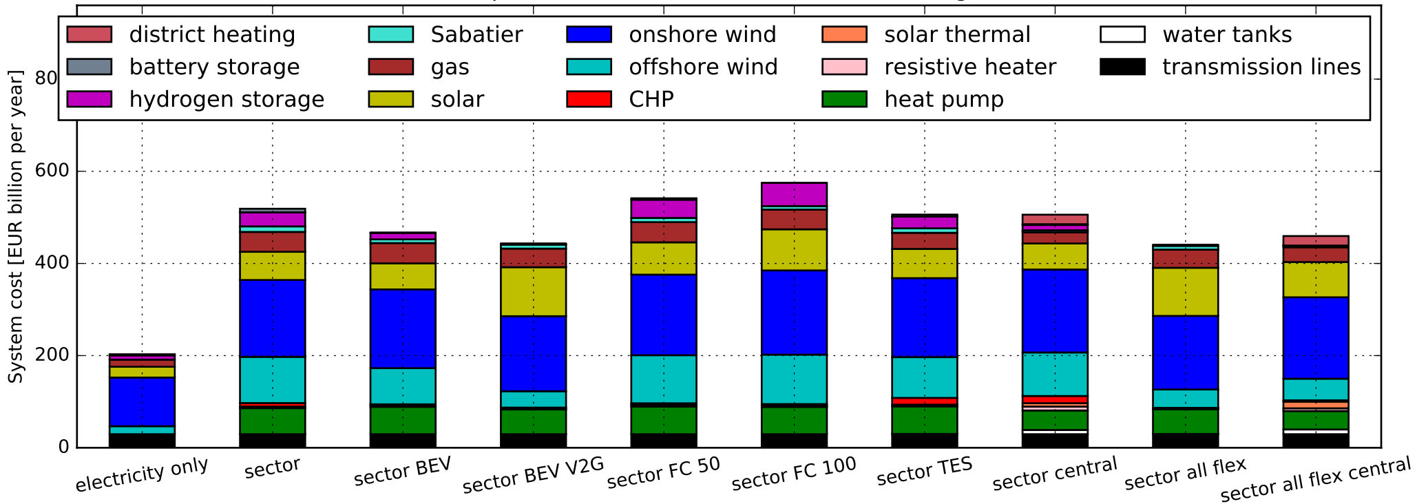
Scenario comparison with 500 TWkm of inter-connecting transmission
