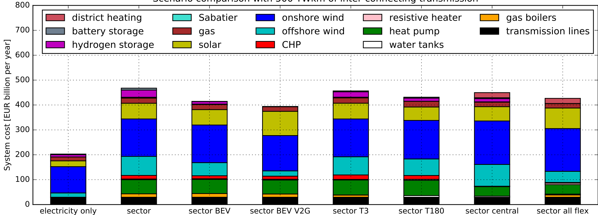
Scenario comparison with 500 TWkm of inter-connecting transmission
