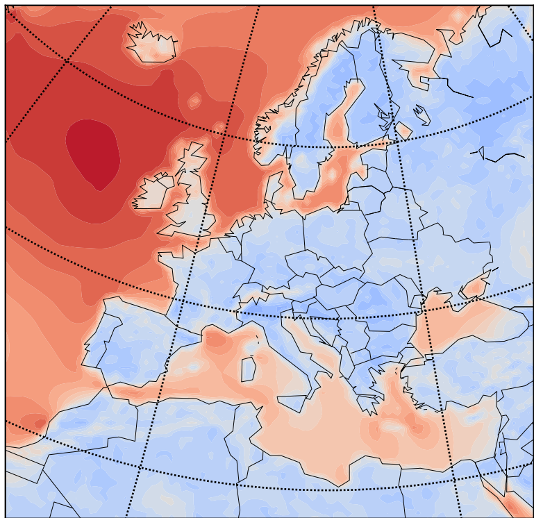
Ensemble Mean - Wind Speed at 10m height - moc
