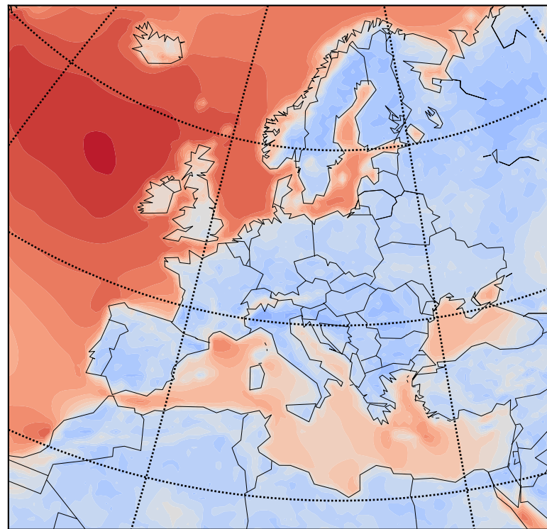
Ensemble Mean - Wind Speed at 10m height - eoc
