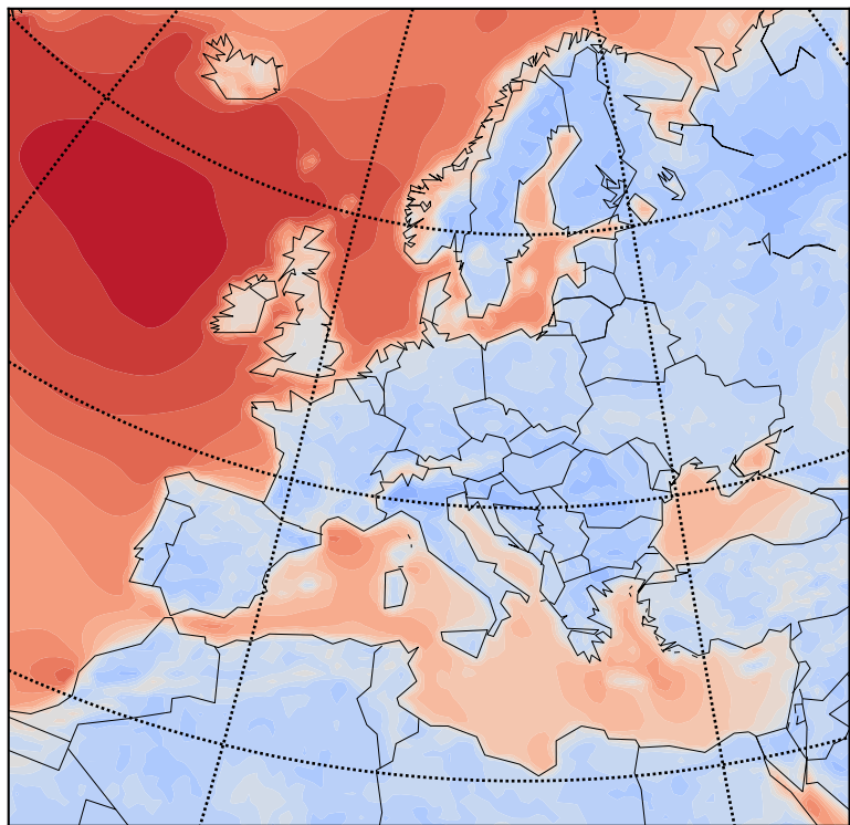
Ensemble Mean - Wind Speed at 10m height - his
