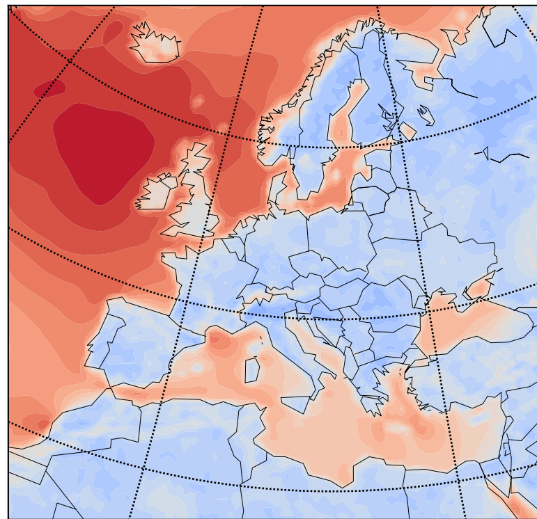
Ensemble Mean - Wind Speed at 10m height - boc
