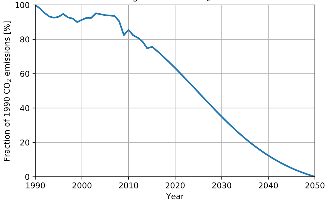
EU28 budget of 48 Gt CO 2 from 2015
