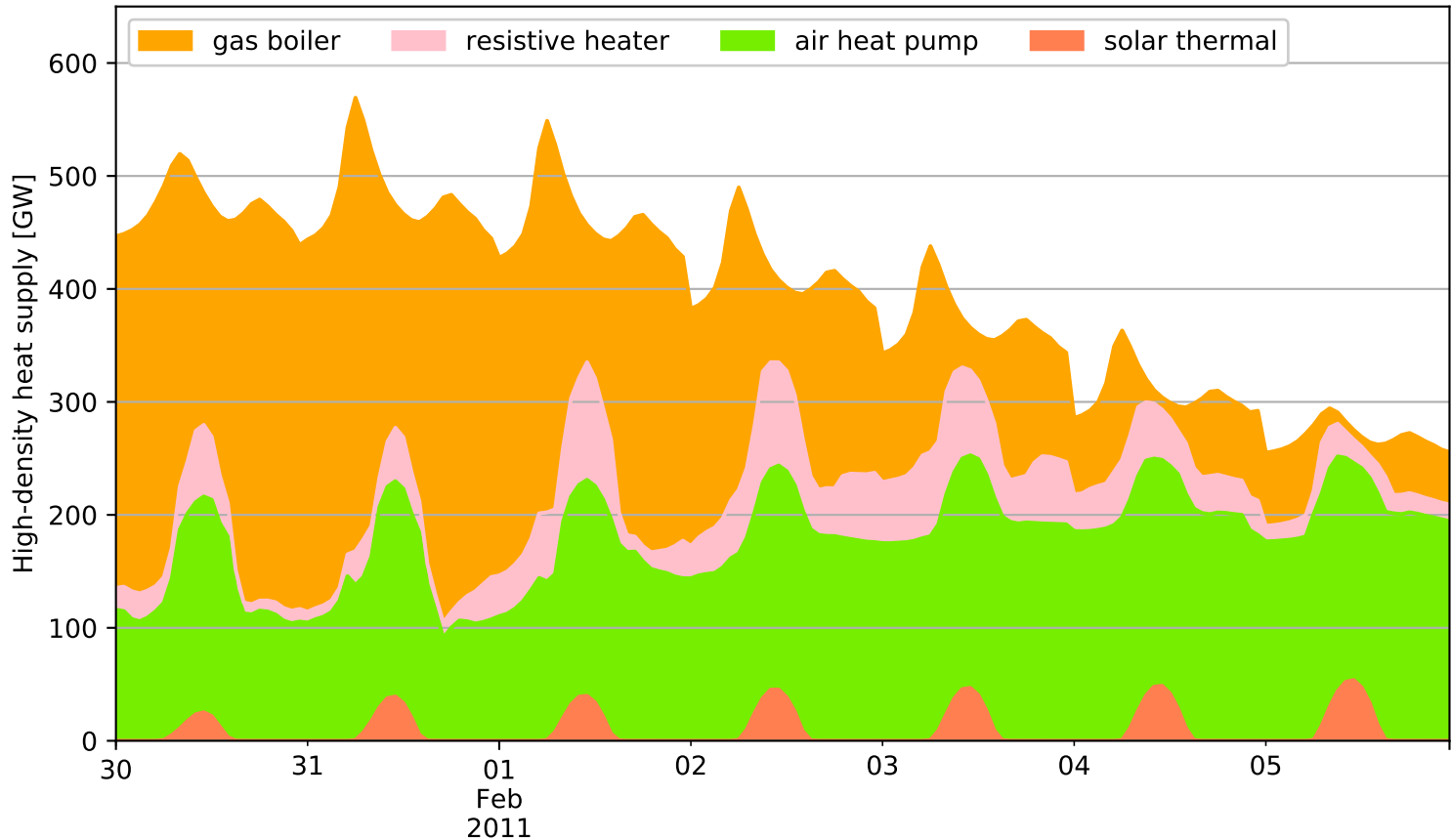
High-density heat supply in Europe for scenario Heating
