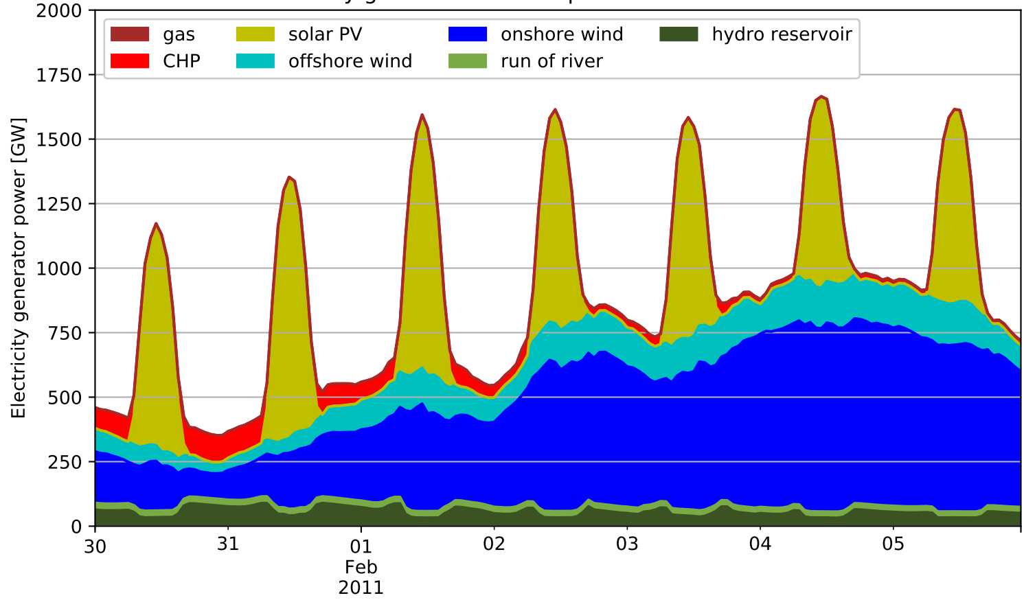
Electricity generation in Europe for scenario Central-TES
