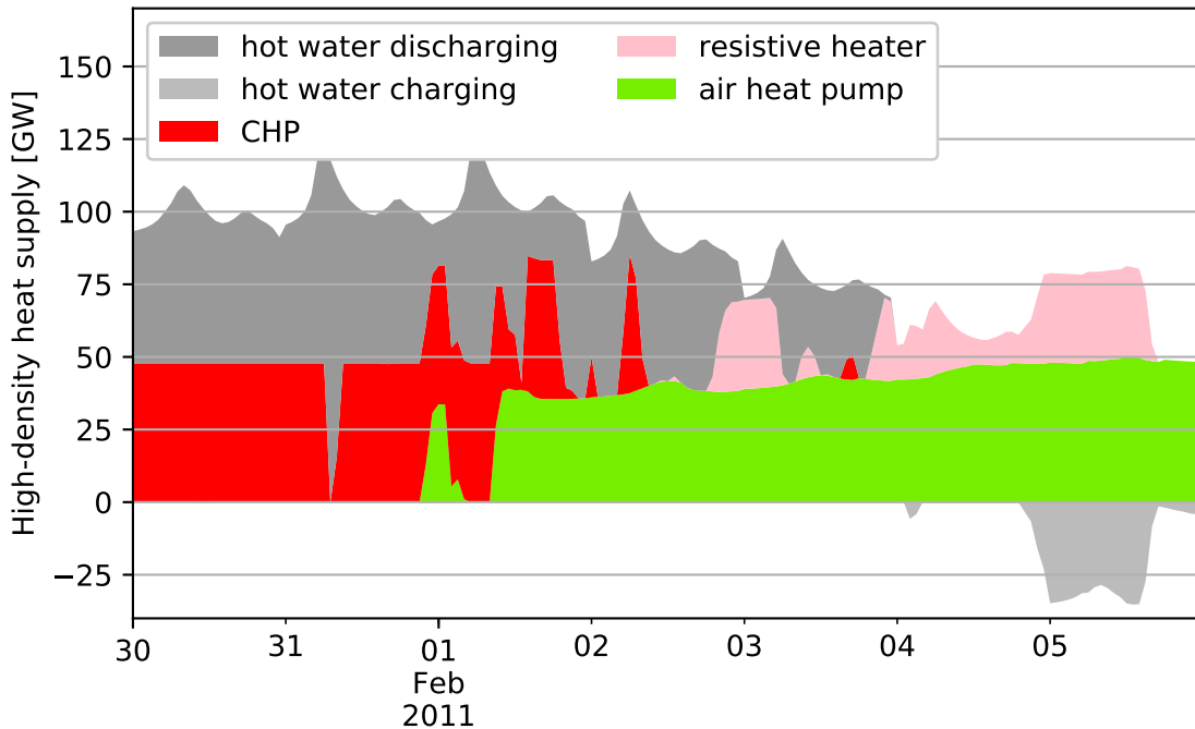
High-density heat supply in DE for scenario Central-TES
