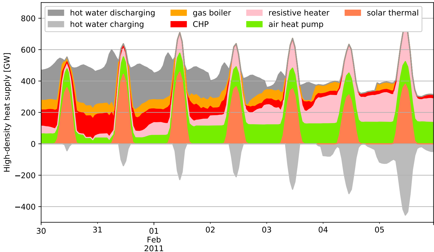
High-density heat supply in Europe for scenario Central-TES
