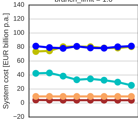
branch_limit = 1.0
