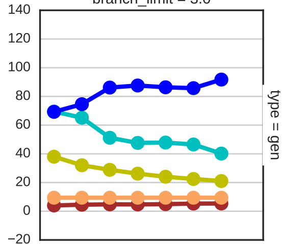
branch_limit = 3.0
