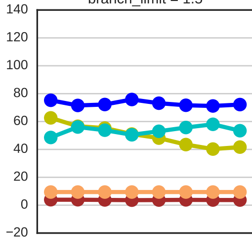
branch_limit = 1.5
