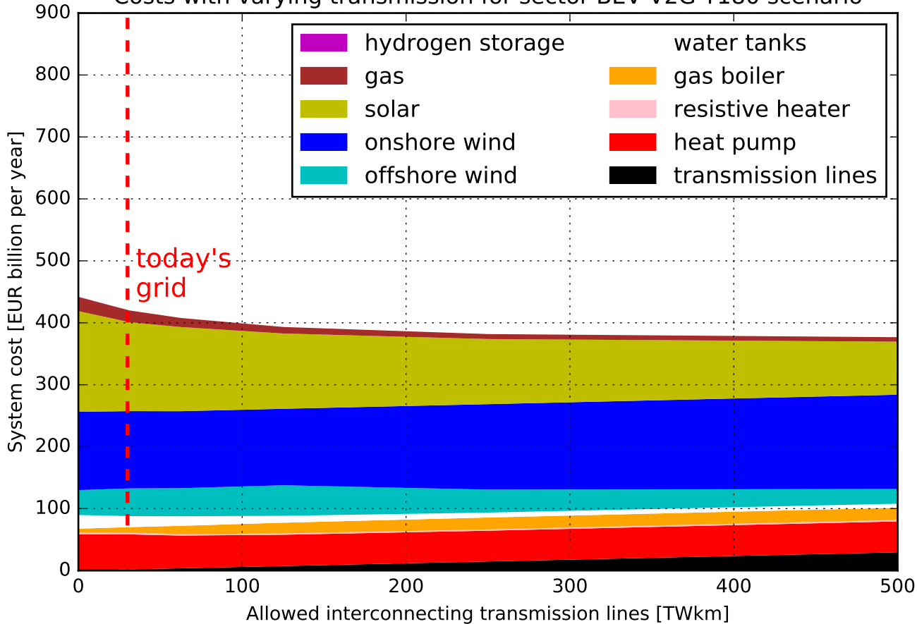
Costs with varying transmission for sector BEV V2G T180 scenario
