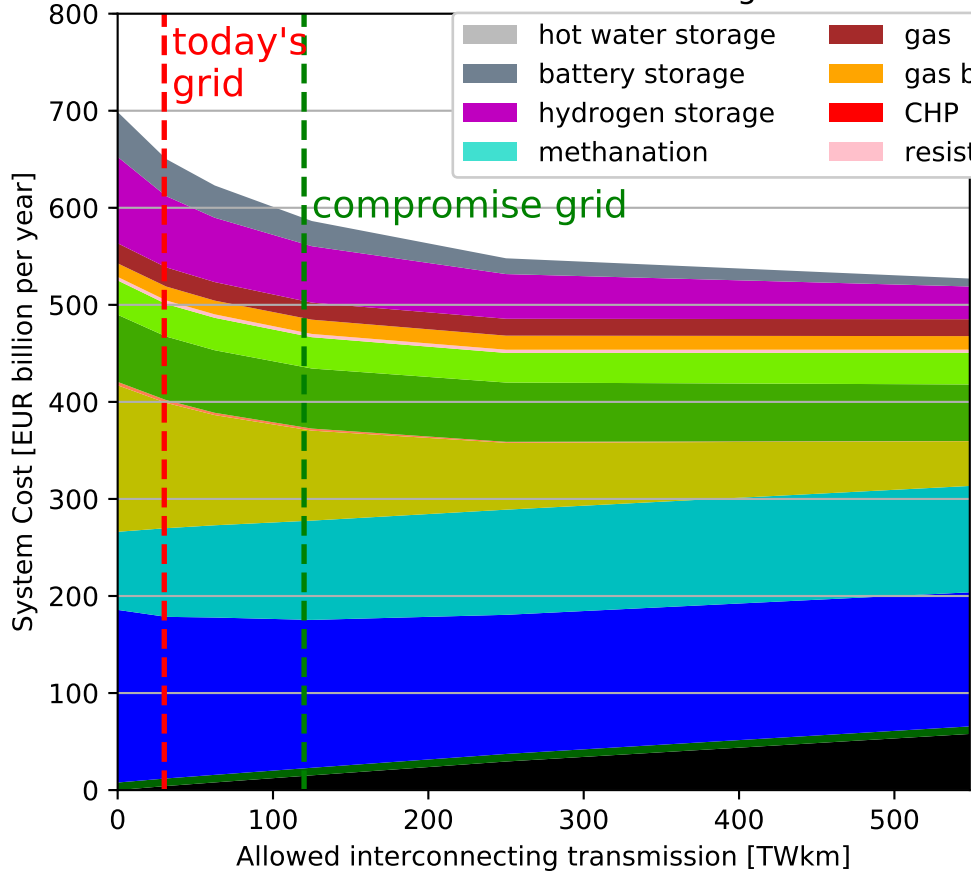
Costs for Scenario Heating
