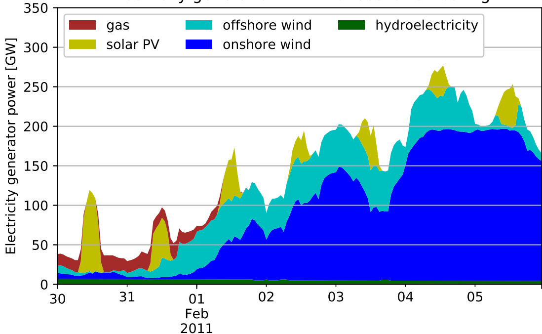
Electricity generation in DE for scenario Heating
