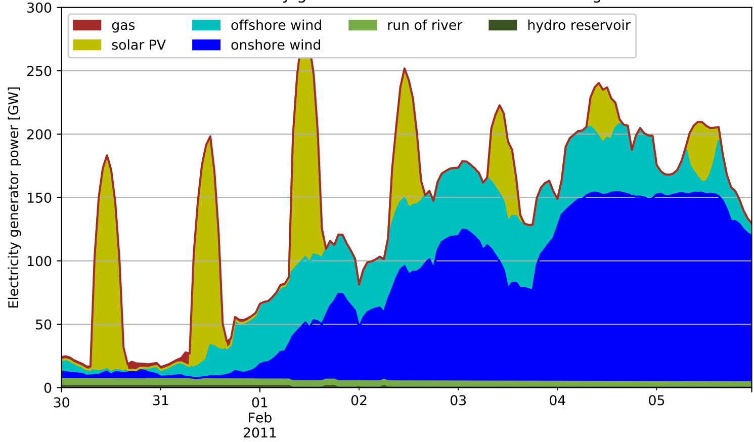
Electricity generation in DE for scenario Heating
