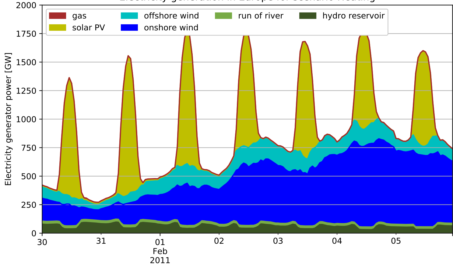
Electricity generation in Europe for scenario Heating
