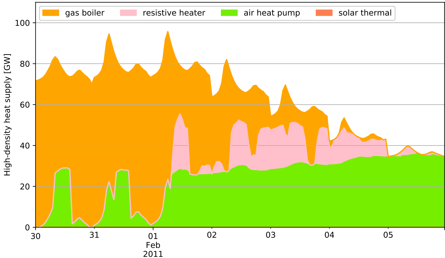
High-density heat supply in DE for scenario Heating
