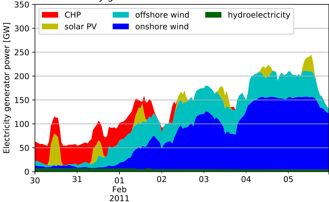
Electricity generation in DE for scenario Central-TES
