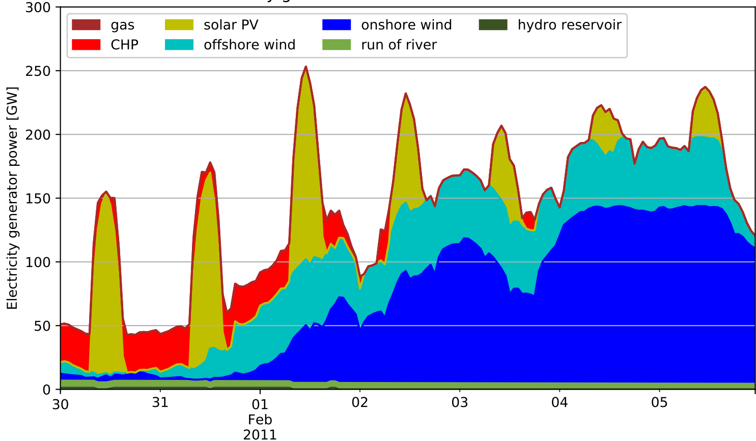
Electricity generation in DE for scenario Central-TES
