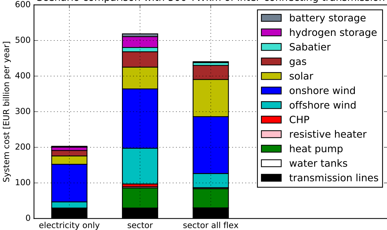
Scenario comparison with 500 TWkm of inter-connecting transmission
