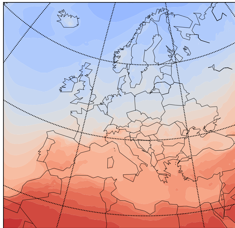
Ensemble Mean - Solar Radiation Influx - boc
