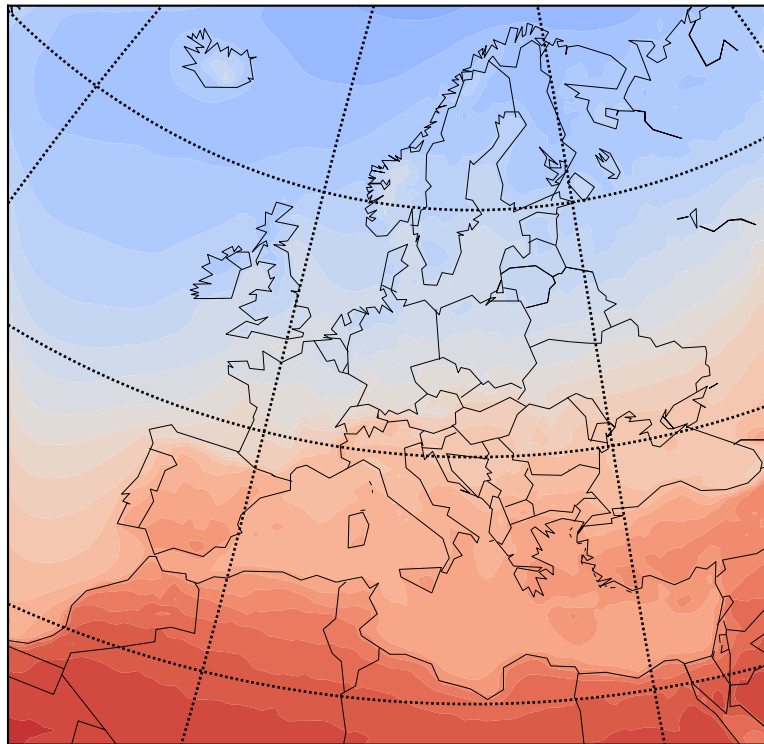
Ensemble Mean - Solar Radiation Influx - moc
