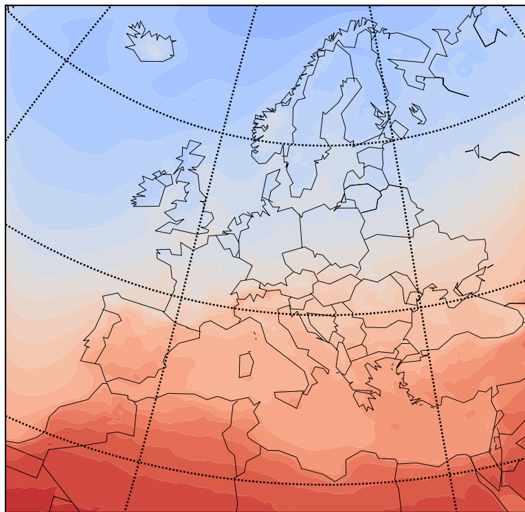
Ensemble Mean - Solar Radiation Influx - his
