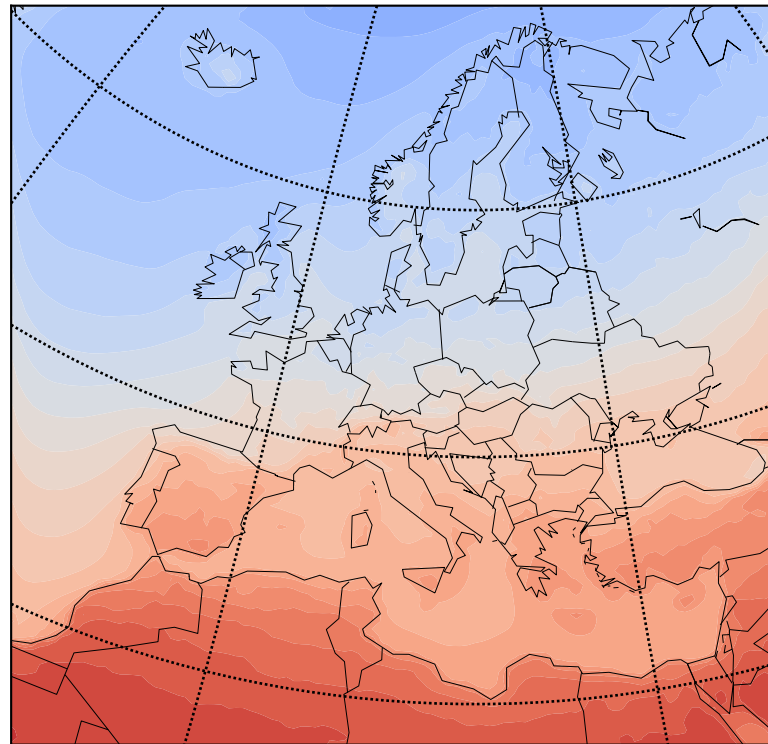
Ensemble Mean - Solar Radiation Influx - eoc
